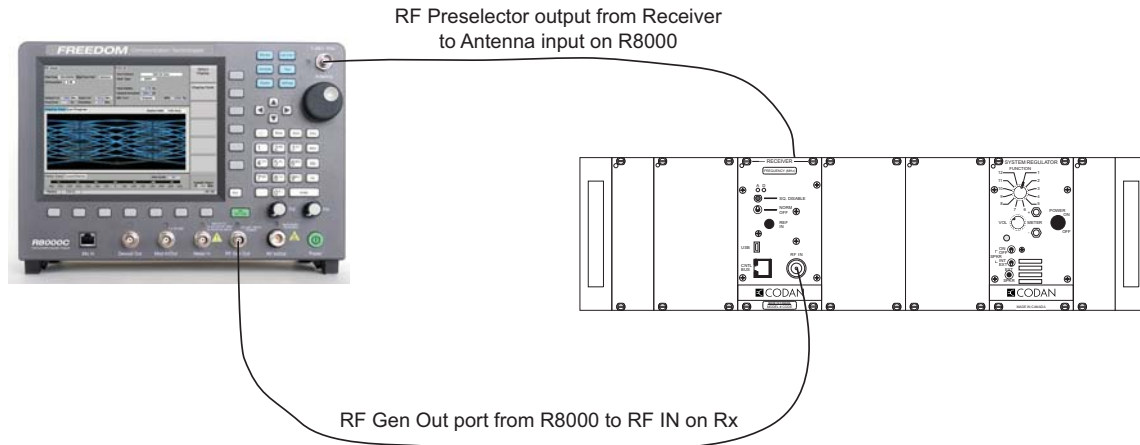
Figure E-15: Receiver RF Preselector Tuning
