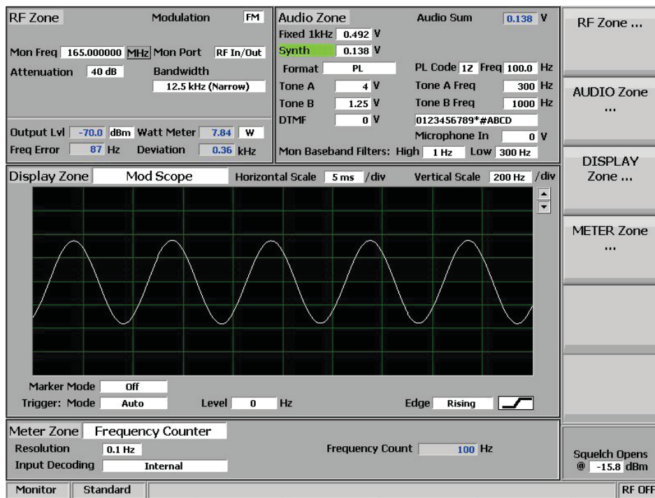
Figure E-30: Transmitter CTCSS Tone and Deviation Measurement
