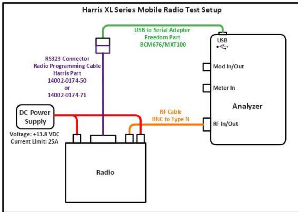
Figure 5-2. XL Series Mobile Test Setup Diagram
